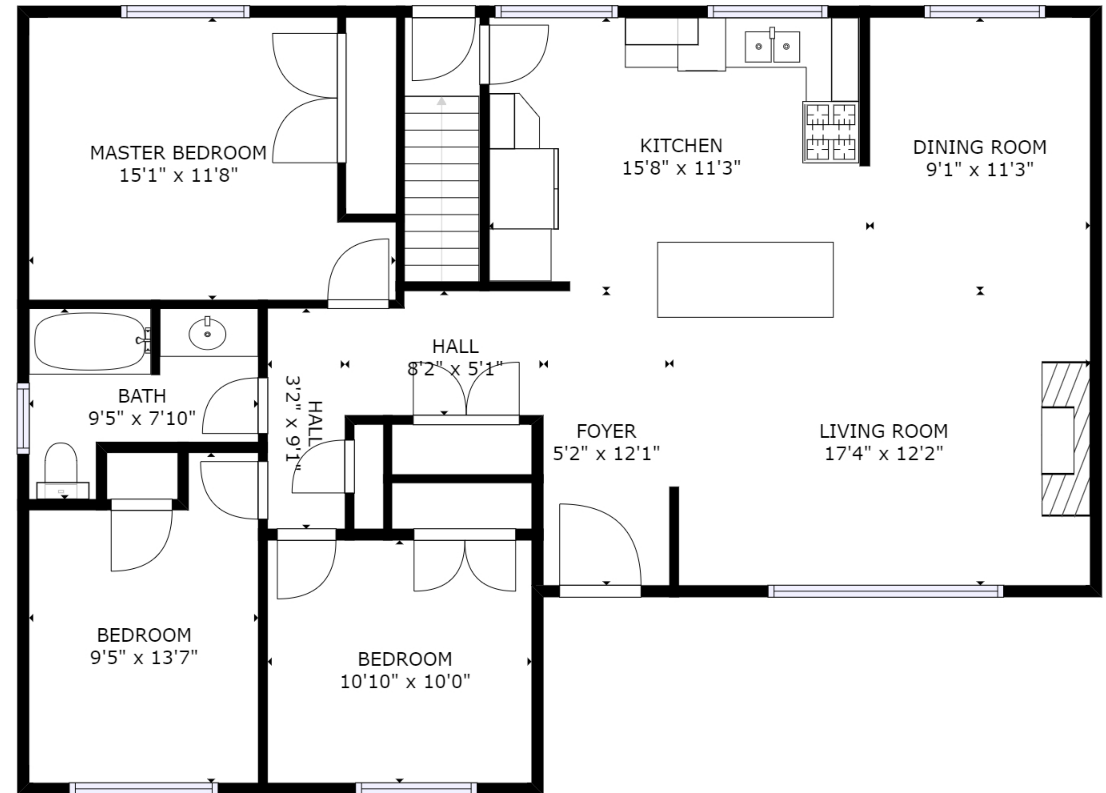
FLOOR 2
